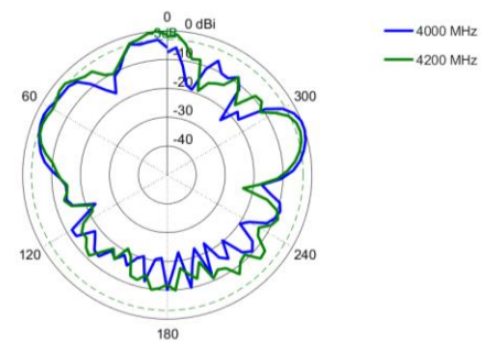
Elevation 2: 4000 – 4200 MHz
