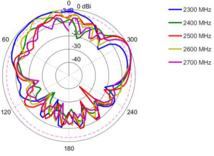
Elevation 1: 2300 – 2700 MHz
