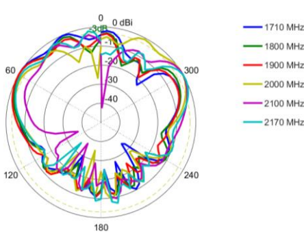
Elevation 2: 1710 – 2170 MHz
